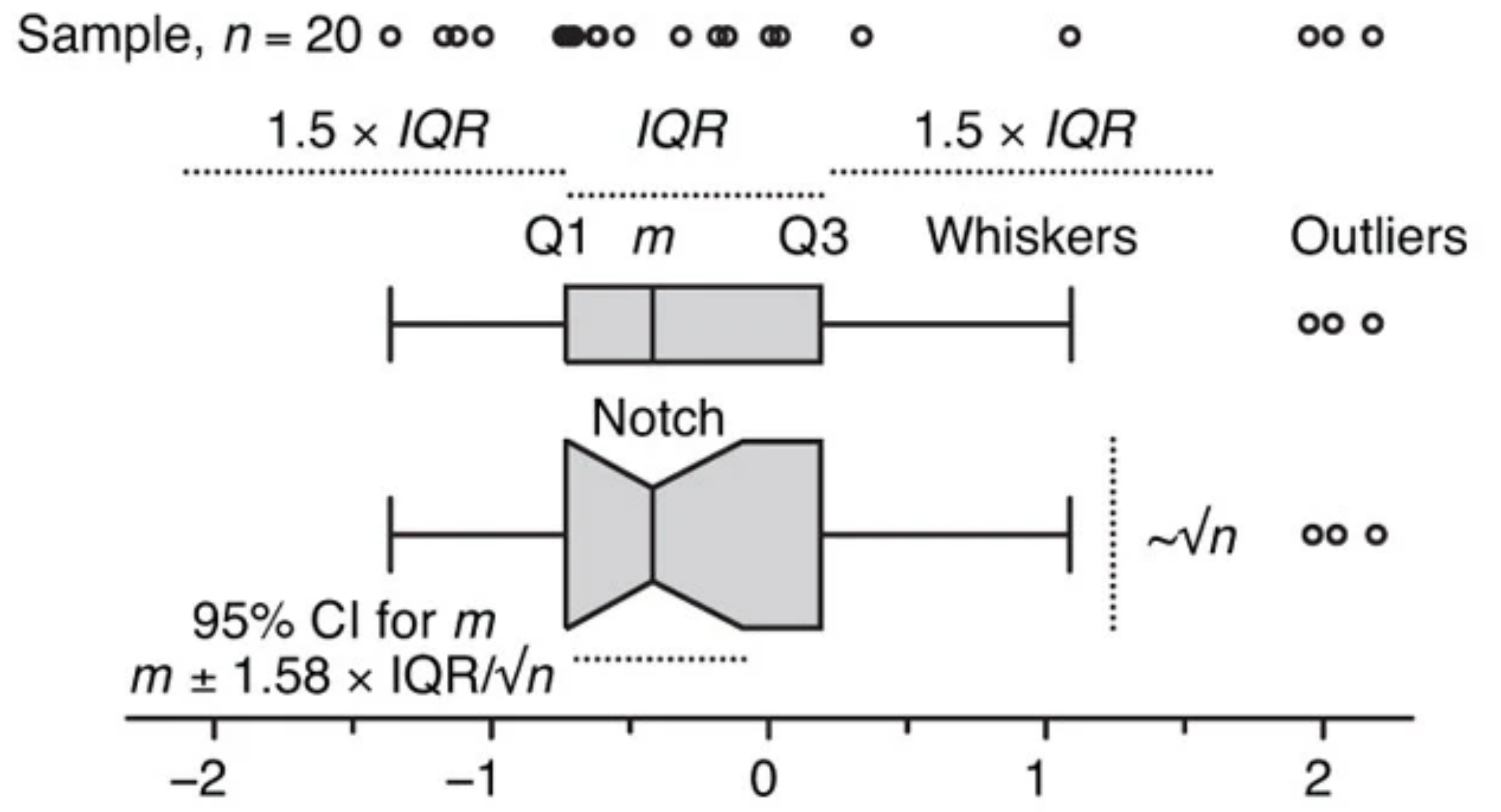
b Construction of a box plot
